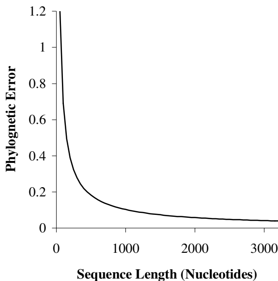
Figure 2 Decreasing power curve relationship between phylogenetic error and sequence length. If sequence length is N , error is approximately proportional to 32 * N^{-0.826} . The slope is steep initially, but decreases rapidly. Between 1000 and 3000 nucleotides, the slope is relatively shallow, and the curve is nearly straight
