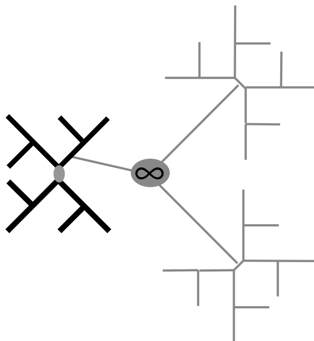
Figure 3 Relationship of doppelgänger trees to focus tree of interest. The shadowy thin grey doppelgänger trees are identical in structure but evolve independently of the focus tree. This is equivalent to being connected to the focus tree by a branch with infinite length. In the bold black focus tree, only reconstruction of the short grey innermost branch was considered.
